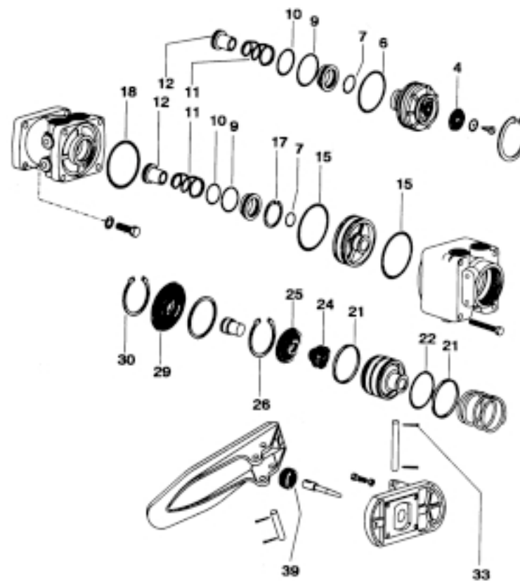
DUAL TREADLE VALVE
