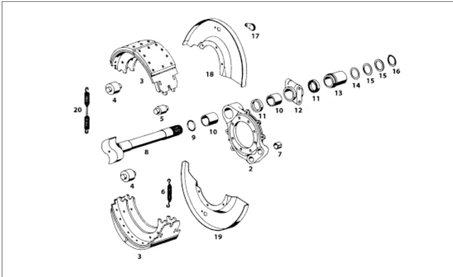
REAR WHEEL BRAKE (BIL)
