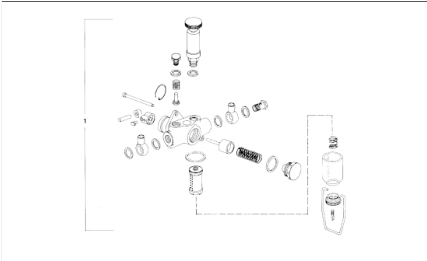
FEED PUMP (MICO)
