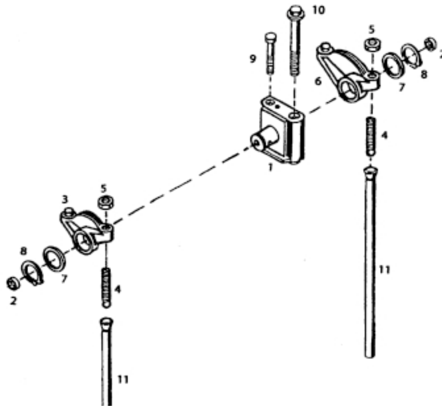
ROCKER LEVER
