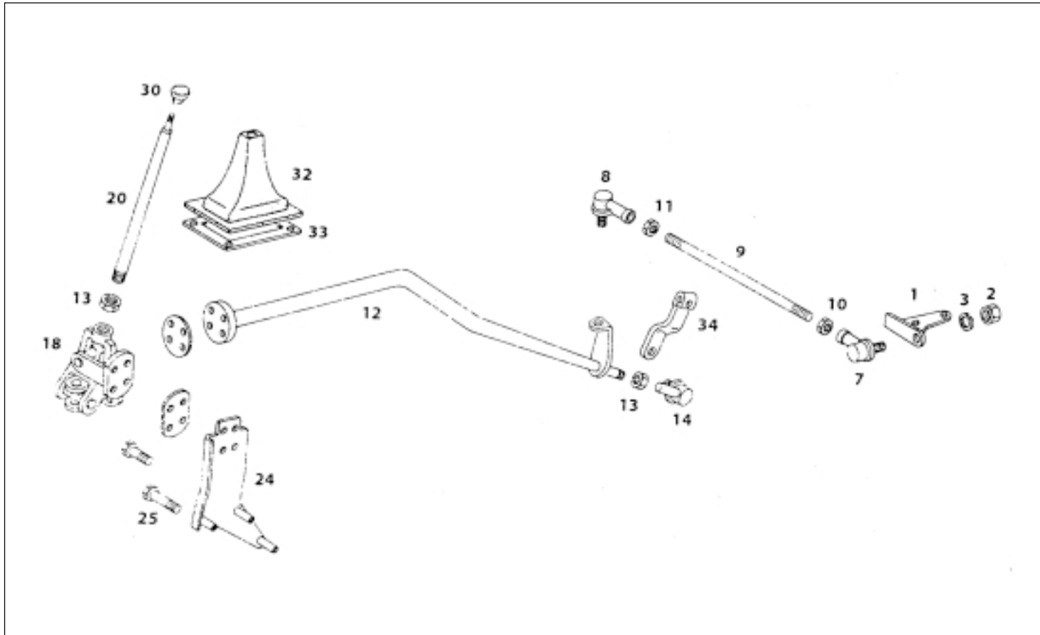
GEAR SHIFTING LINKAGE (LPO)
