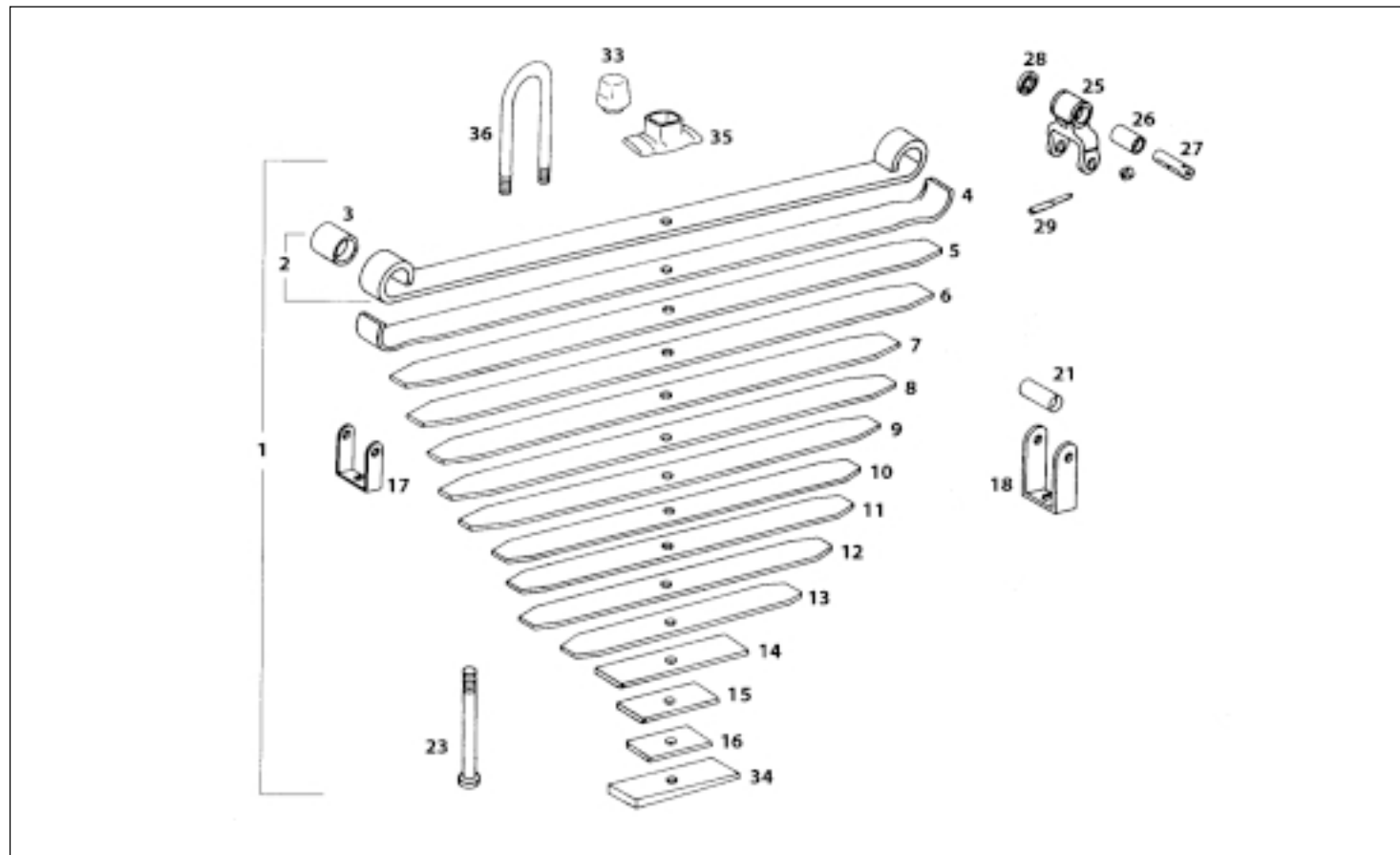
FRONT SPRING SUSPENSION (LPO)
