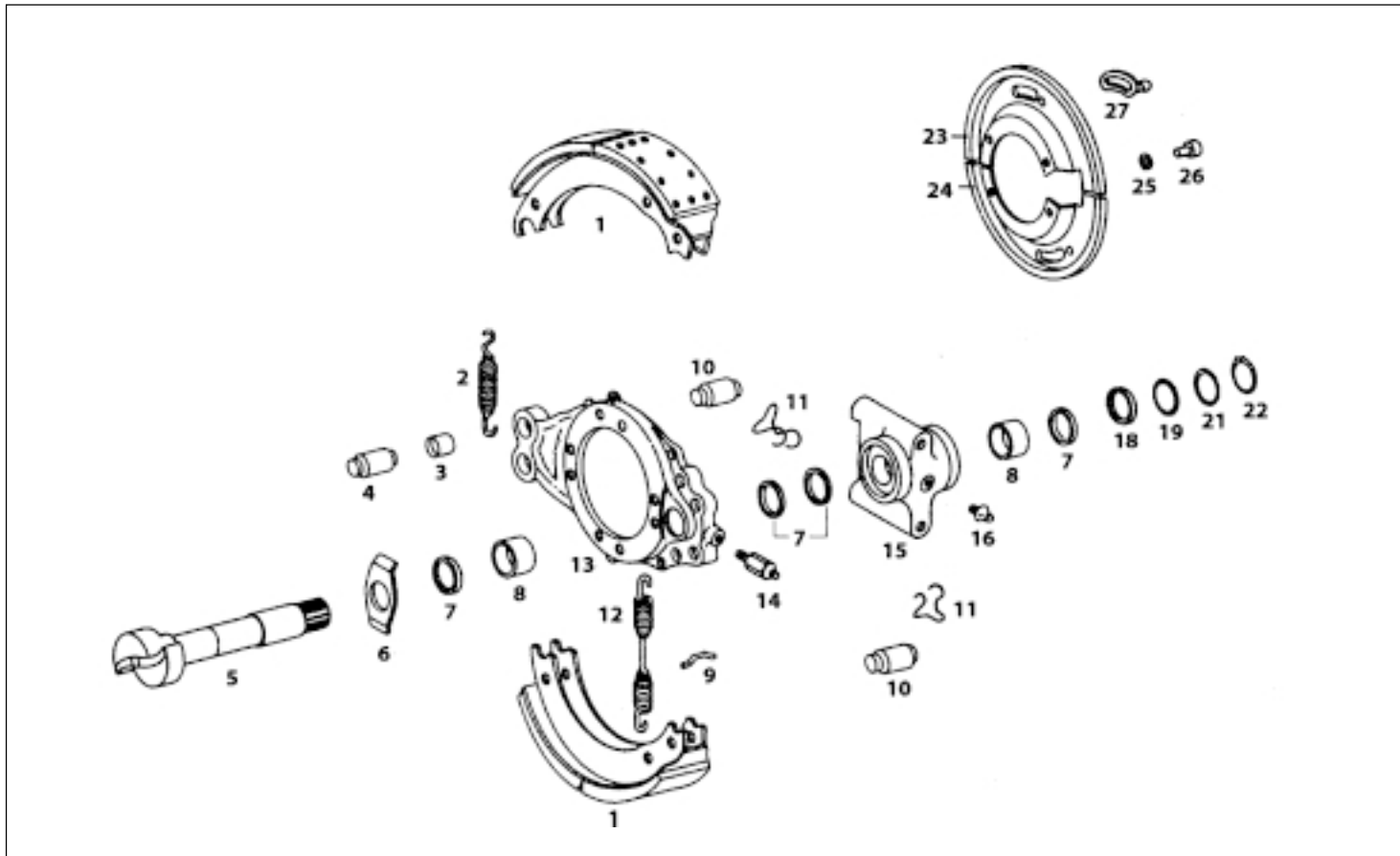
REAR WHEEL BRAKE (AAL)
