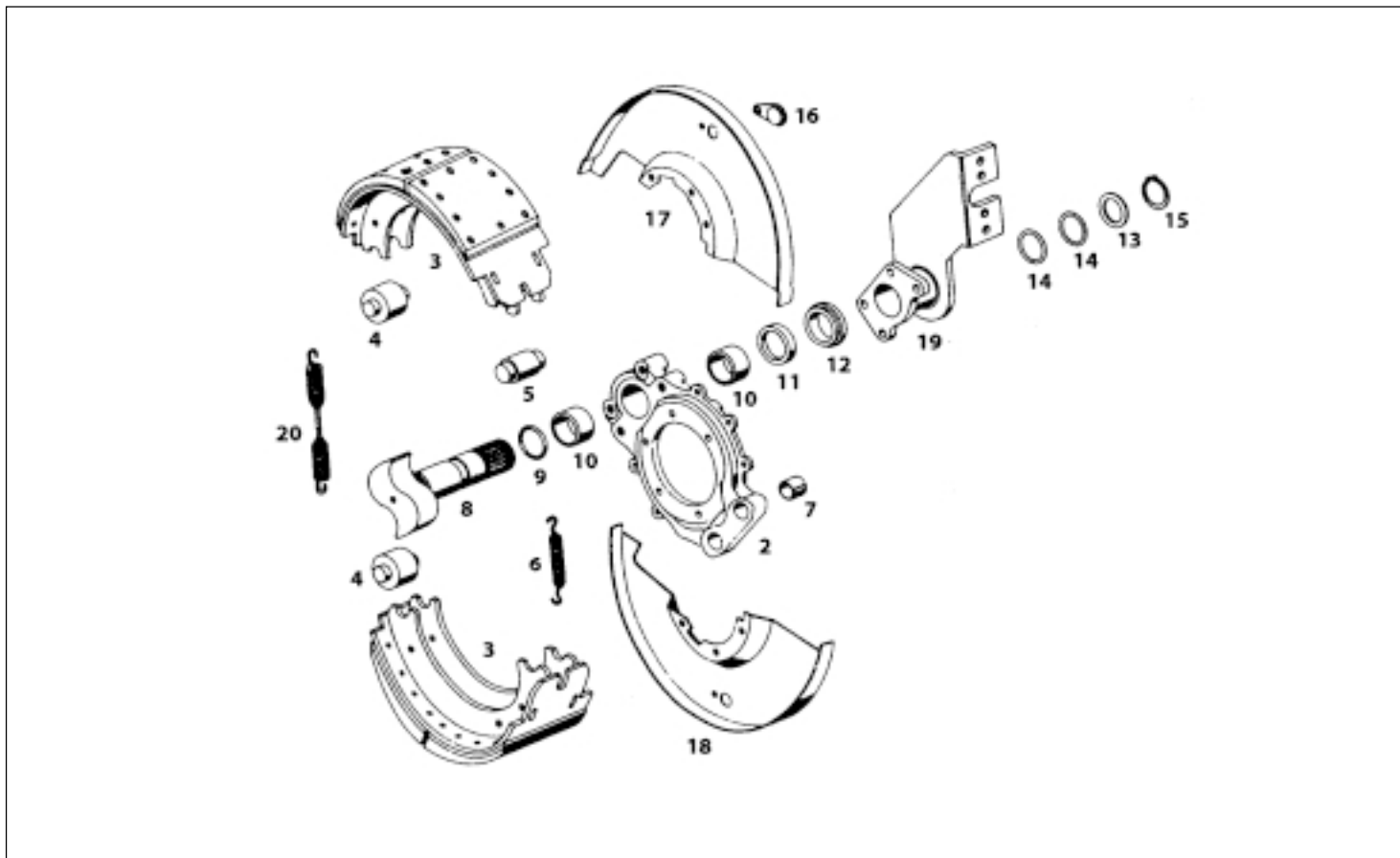
FRONT WHEEL BRAKE (BIL)
