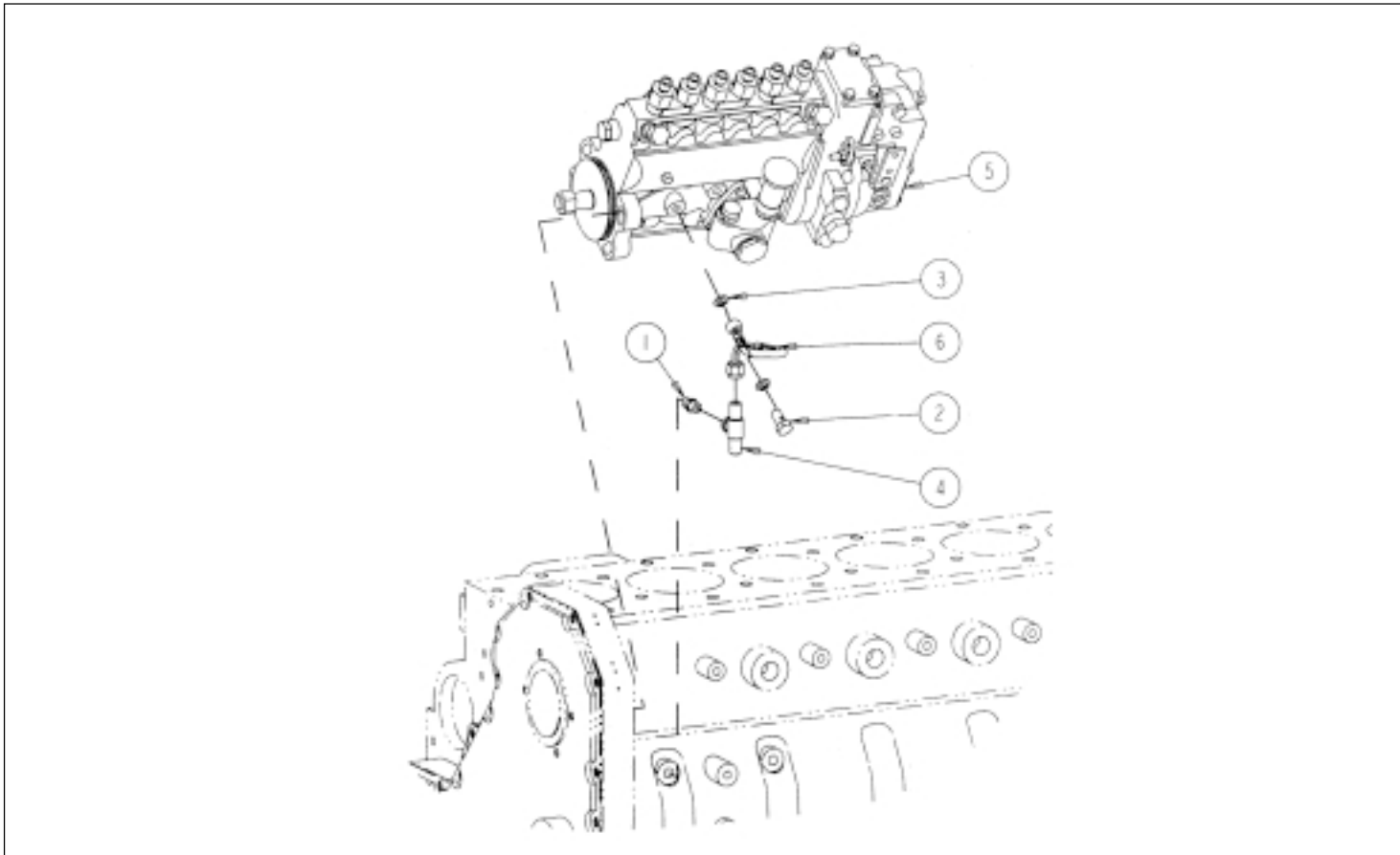
FUEL PUMP BASE (IN LINE FIP)
