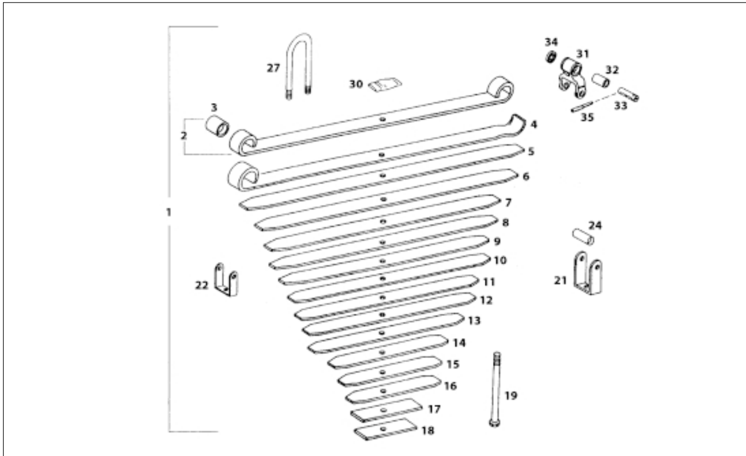
REAR SPRING SUSPENSION (LPO)
