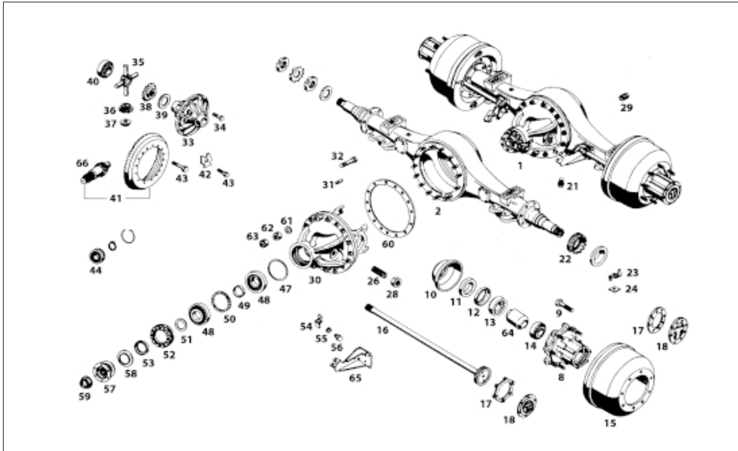
REAR AXLE (RA 108 RR)
