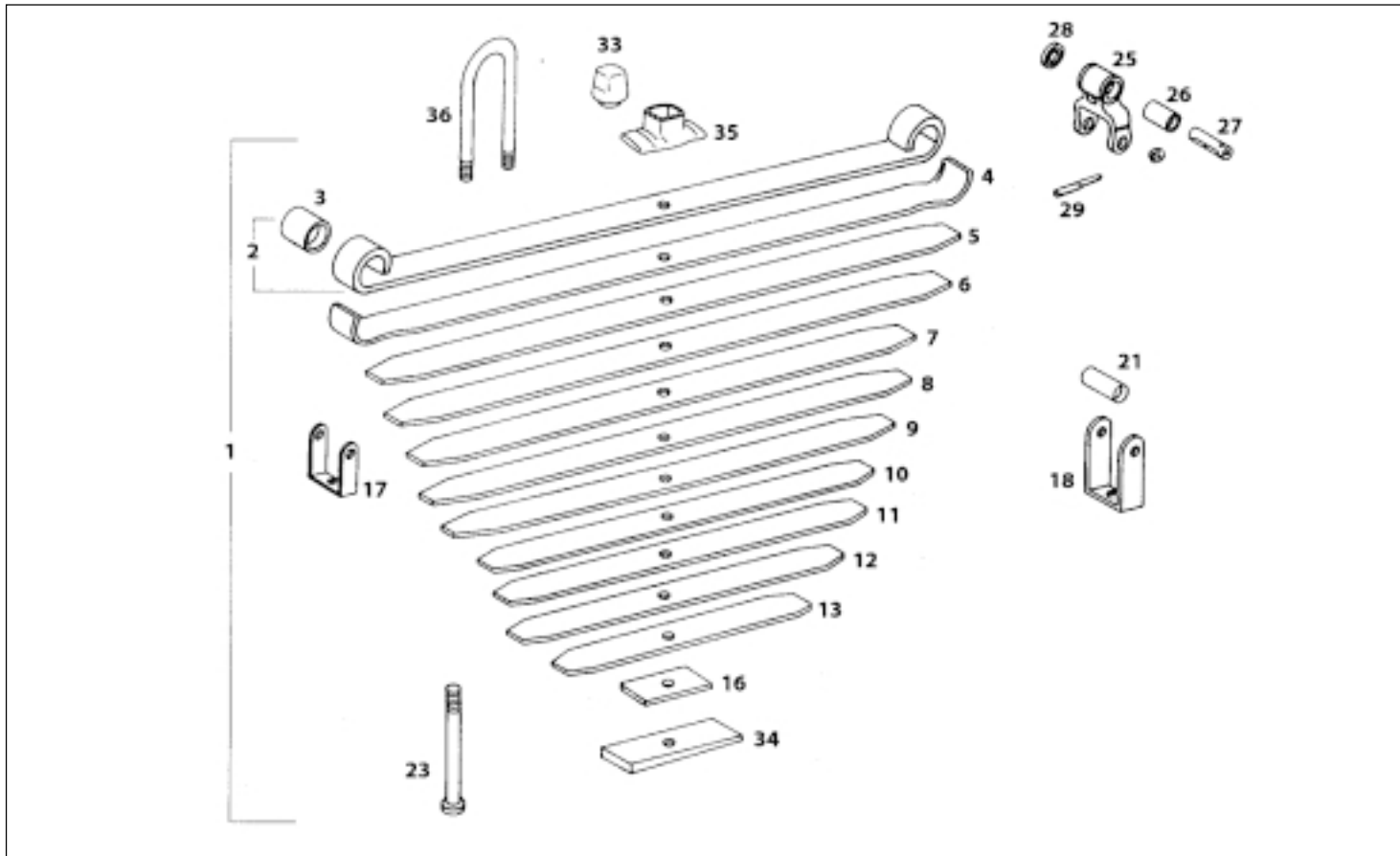
FRONT SPRING SUSPENSION (LP)
