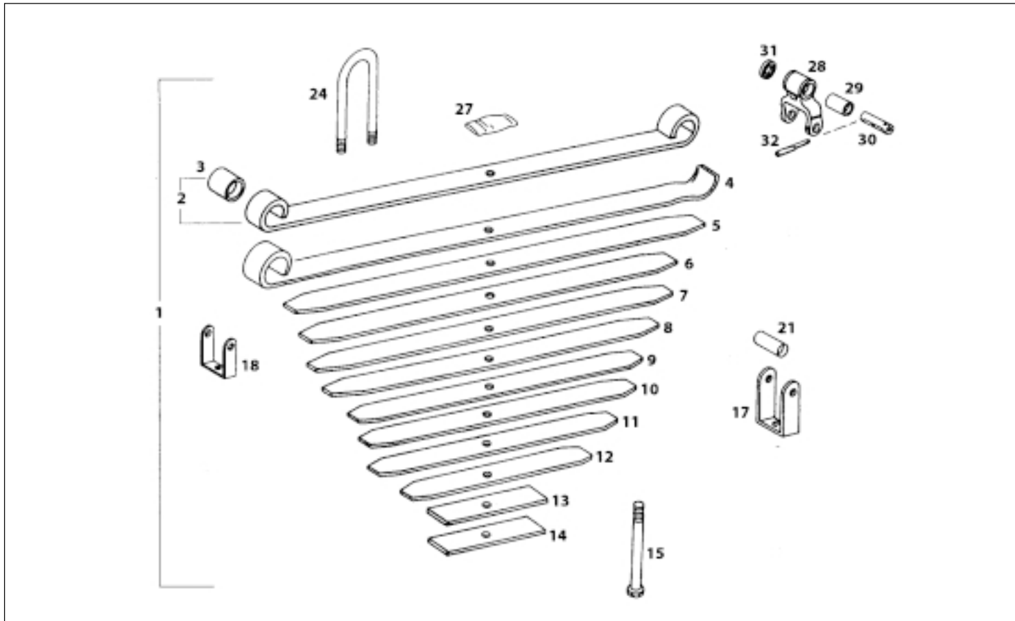
REAR SPRING SUSPENSION (LP)
