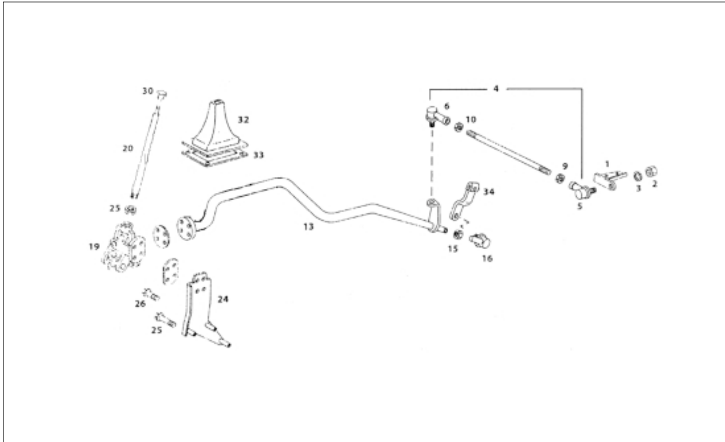
GEAR SHIFTING LINKAGE (LP)
