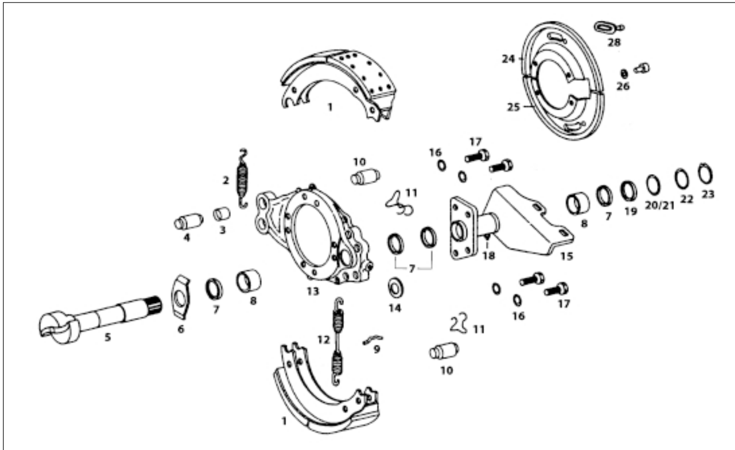
FRONT WHEEL BRAKE (AAL)
