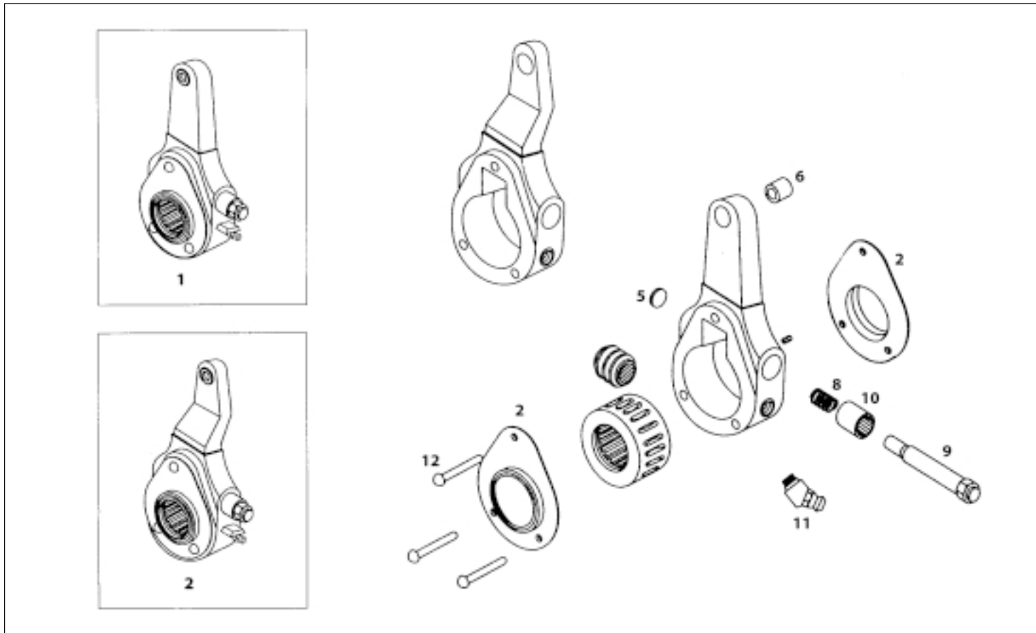
SLACK ADJUSTER (FRONT AND REAR)
