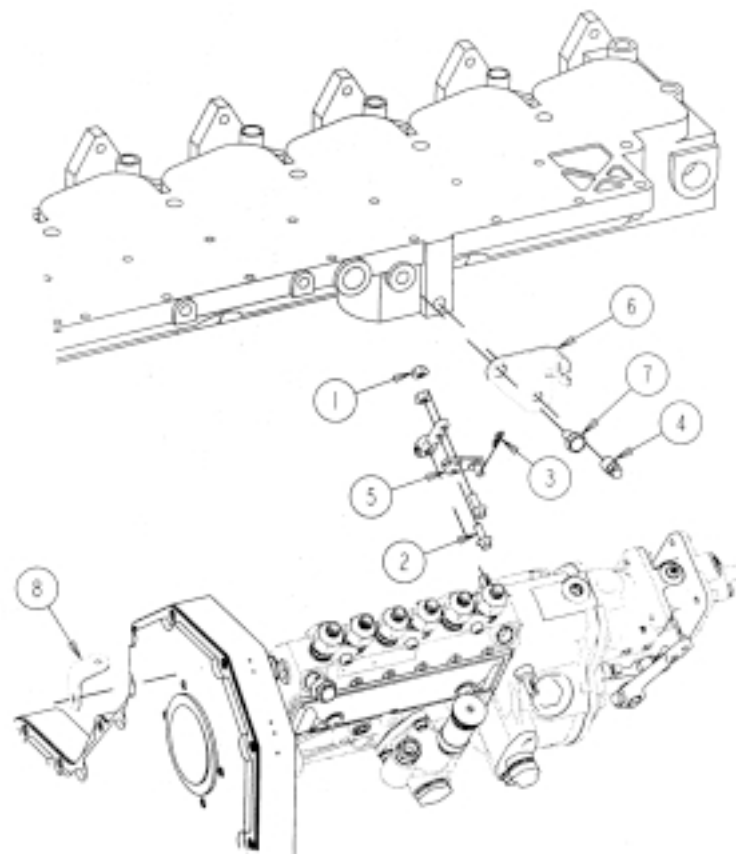
LEVER FUEL SHUT OFF
